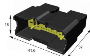
适配A型卡扣 / Mating Type A Clip
